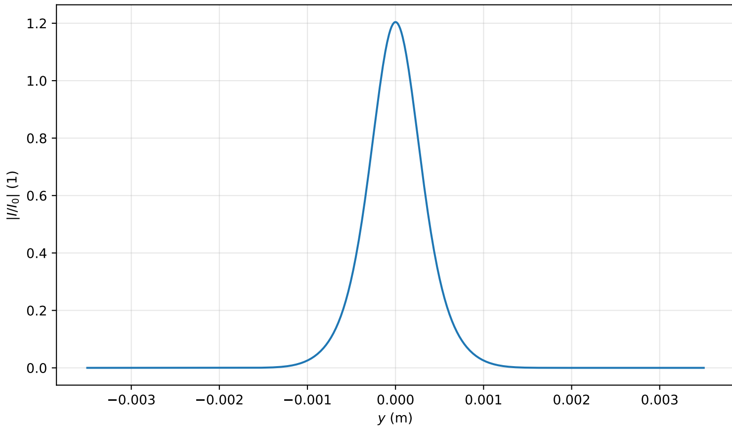
Intensity profile I(x=0, y, z=1.035)/I_0 , P_{in}=0.7P_{cr} , artificial time
